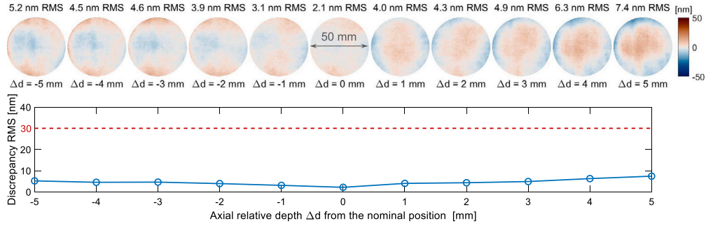
Fig. 7. The reconstruction of a flat mirror is insensitive to the depth change within a 10 mm range using the CPMD technique. The top panel displays the discrepancy maps of the measurements at different depths, and the bottom plot shows the RMS values of the discrepancies v.s. the axial relative depth from the nominal position.
