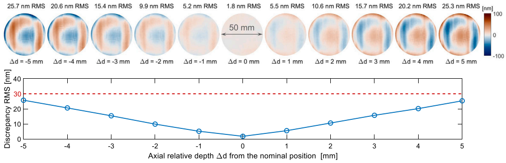
Fig. 9. The reconstruction of a spherical mirror ( \text{RoC} \approx 200 mm) is insensitive to the depth change within a 10 mm range using the CPMD technique. The top panel displays the discrepancy maps of the measurements at different depths, and the bottom plot shows the RMS values of discrepancies v.s. the axial depth from the nominal position.
